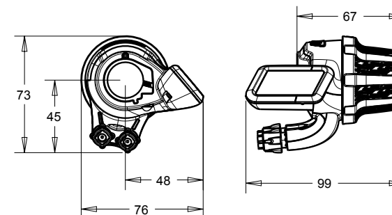
C8s controller
