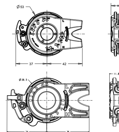
Nfinity Naben-Interface
